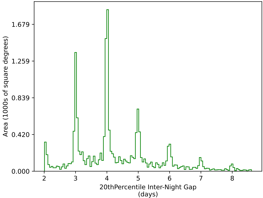
too_elab_heavy_r32_d3_gz_v3.4_10yrs WFD g band: 20thPercentile Inter-Night Gap
