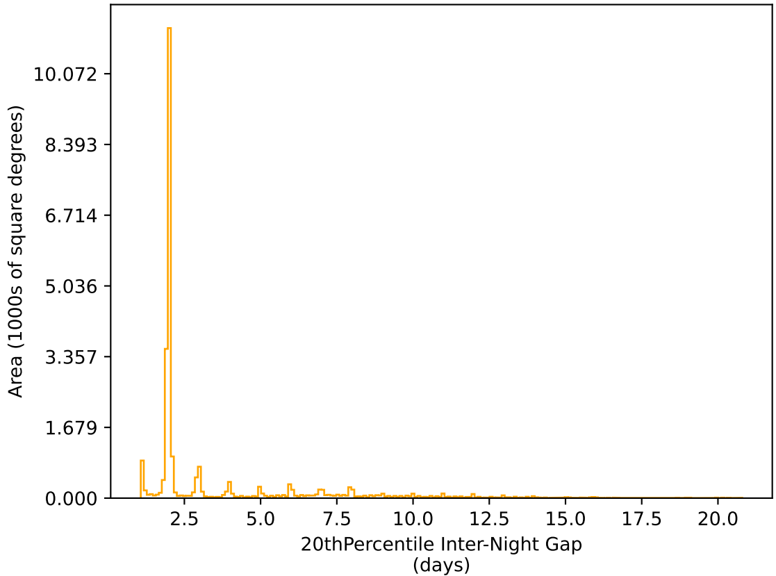
too_elab_heavy_r32_d3_gz_v3.4_10yrs All sky r band: 20thPercentile Inter-Night Gap
