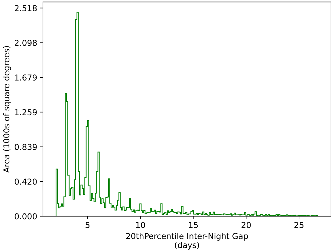
too_elab_heavy_r32_d3_gz_v3.4_10yrs All sky g band: 20thPercentile Inter-Night Gap
