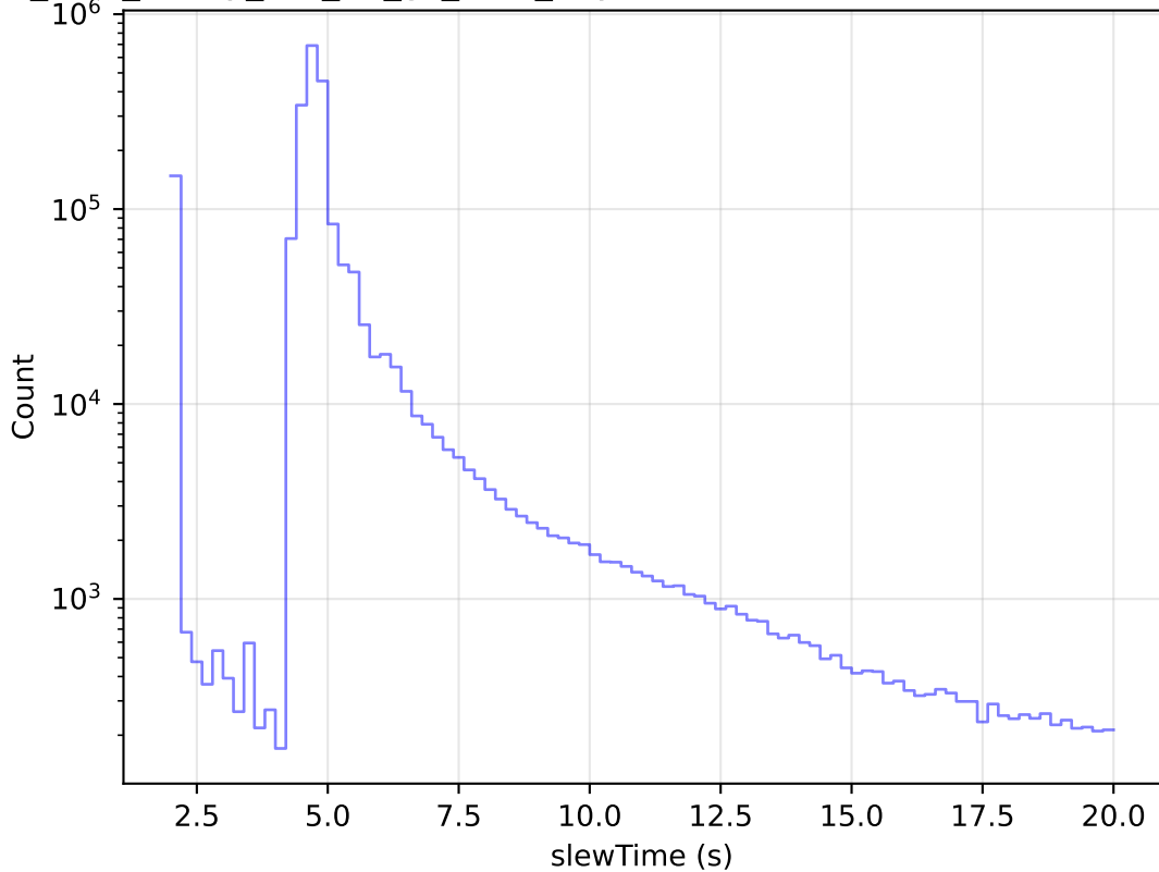
too_elab_heavy_r32_d3_gz_v3.4_10yrs All visits: Zoom Slew Time Histogram
