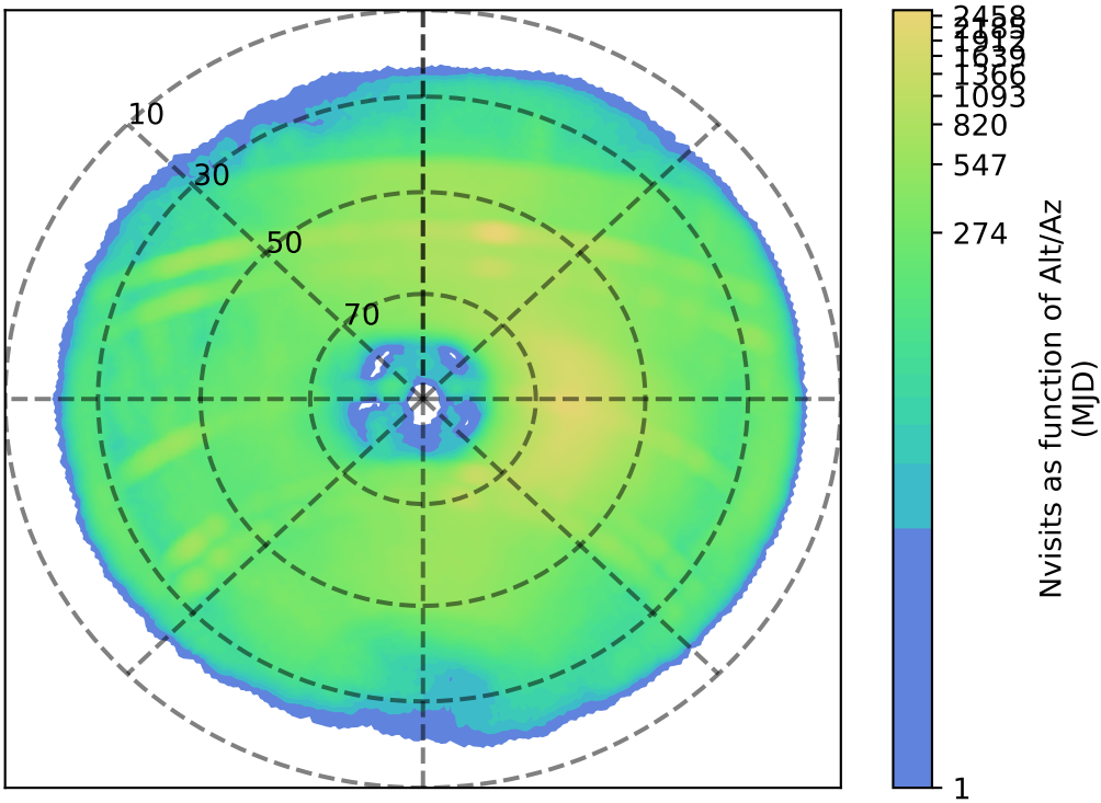
too_elab_heavy_r32_d3_gz_v3.4_10yrs z: Nvisits as function of Alt/Az
