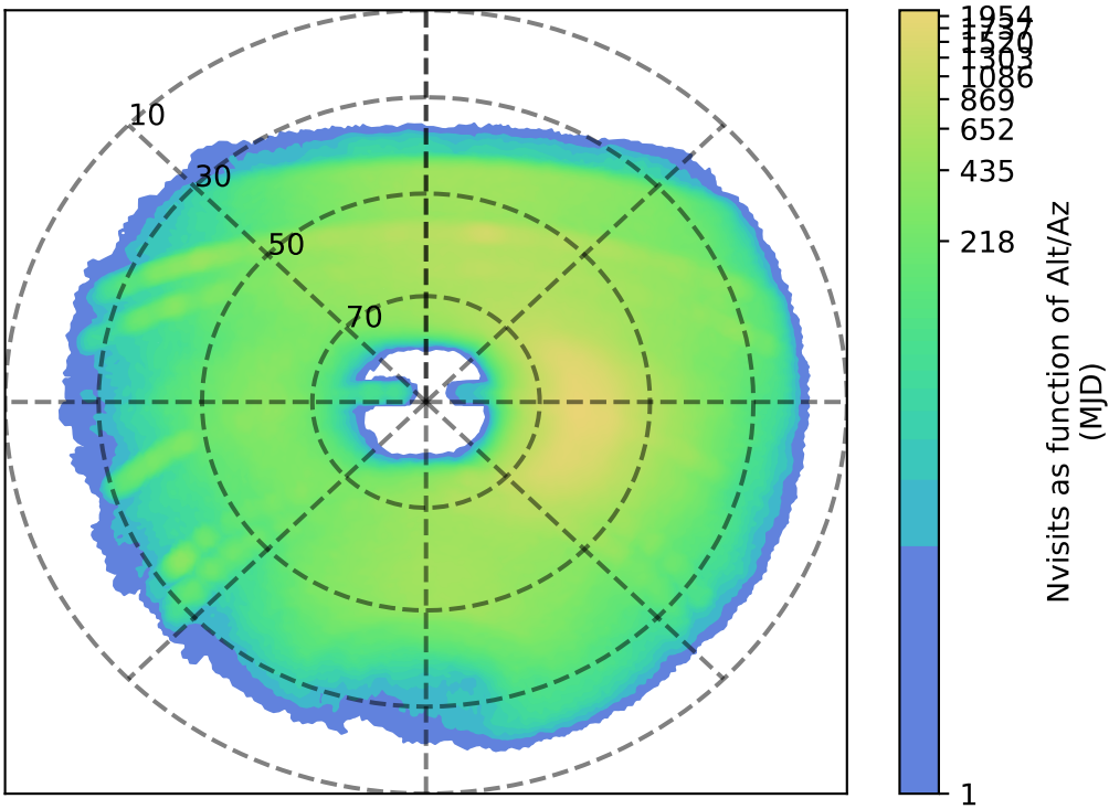
too_elab_heavy_r32_d3_gz_v3.4_10yrs y: Nvisits as function of Alt/Az
