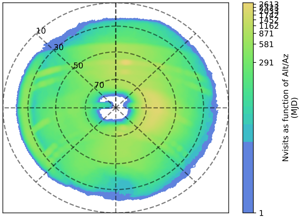
too_elab_heavy_r32_d3_gz_v3.4_10yrs r: Nvisits as function of Alt/Az
