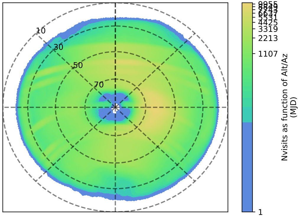
too_elab_heavy_r32_d3_gz_v3.4_10yrs : Nvisits as function of Alt/Az
