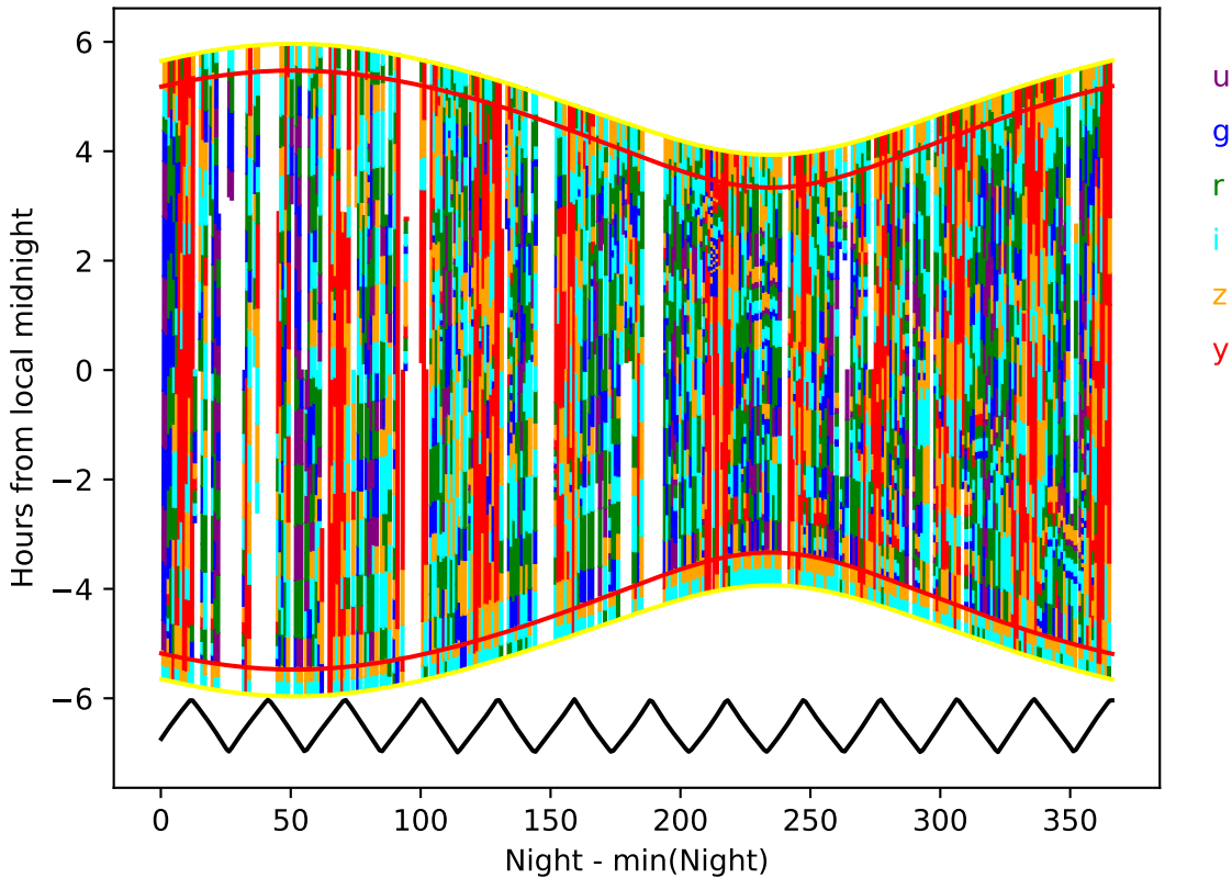
too_elab_heavy_r32_d3_gz_v3.4_10yrs_year 0-1: Hourglass
