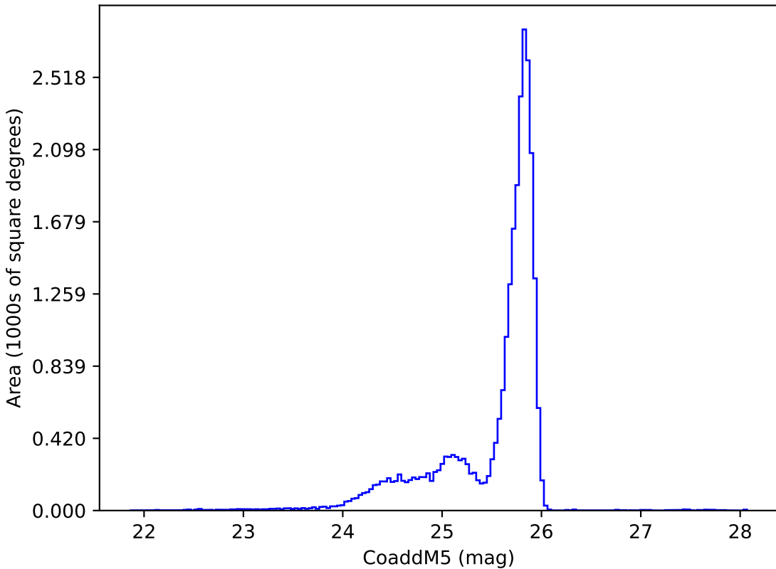
too_elab_heavy_r32_d3_gz_v3.4_10yrs z: CoaddM5
