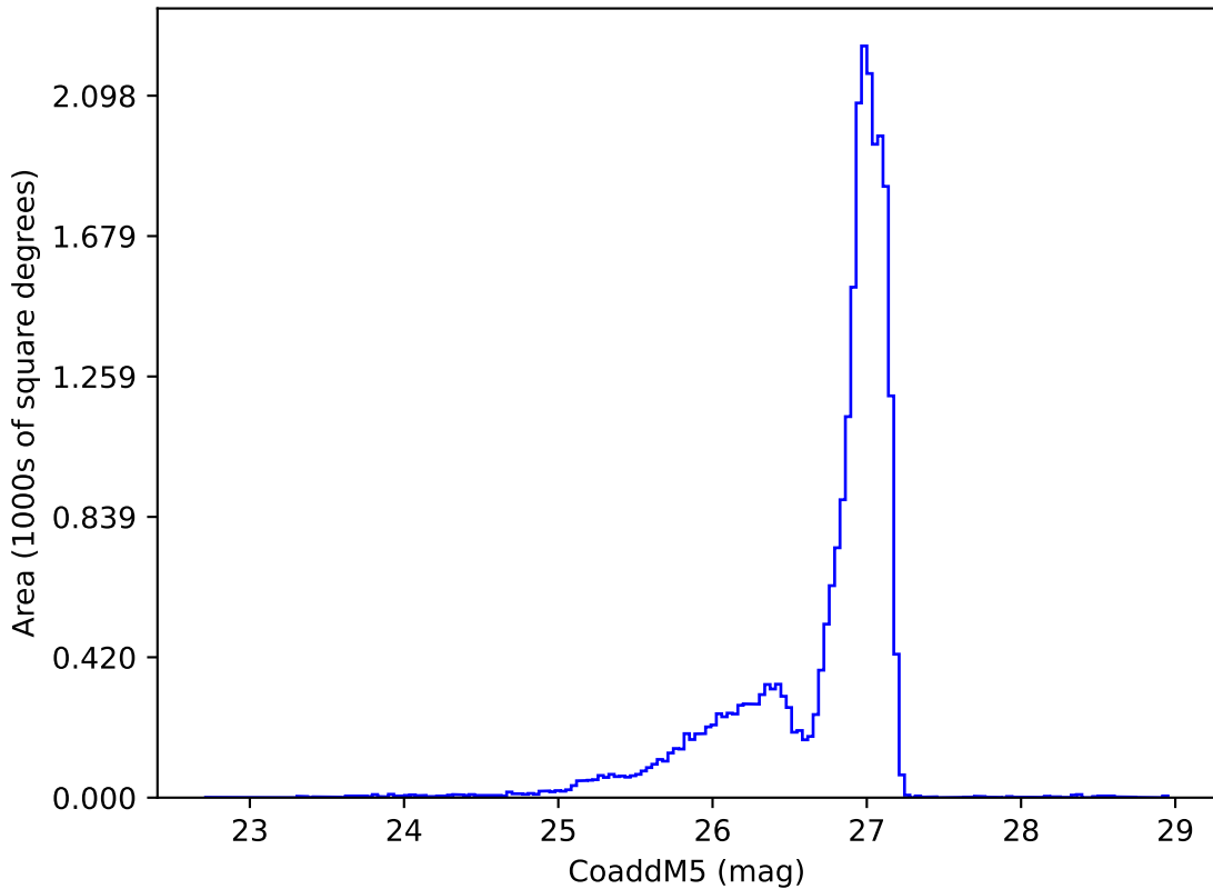
too_elab_heavy_r32_d3_gz_v3.4_10yrs r: CoaddM5
