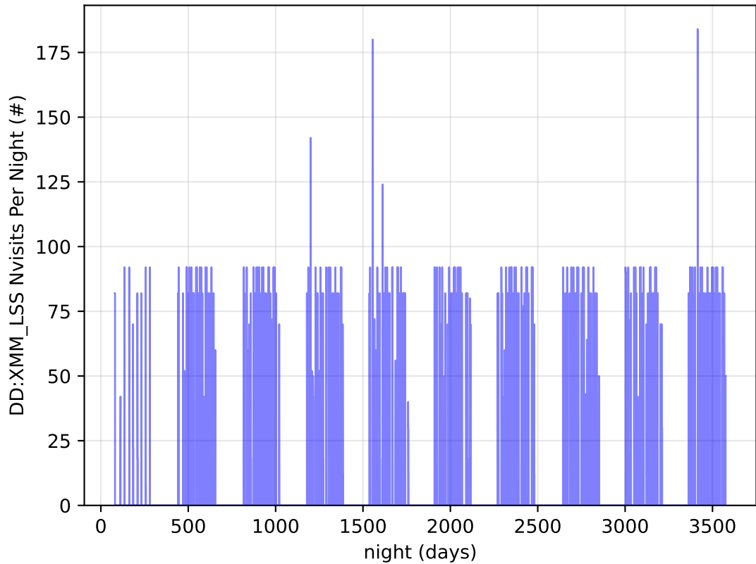
too_elab_heavy_r32_d3_gz_v3.4_10yrs all bands: DD:XMM_LSS Nvisits Per Night
