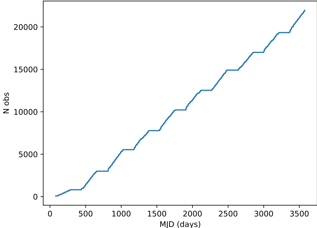
too_elab_heavy_r32_d3_gz_v3.4_10yrs all bands: DD:XMM_LSS Cumulative NVisits
