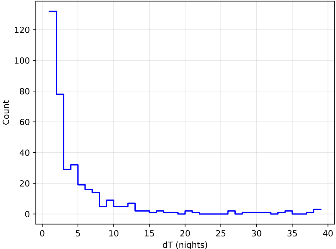
too_elab_heavy_r32_d3_gz_v3.4_10yrs all bands: DD:WFD Delta Nights Histogram
