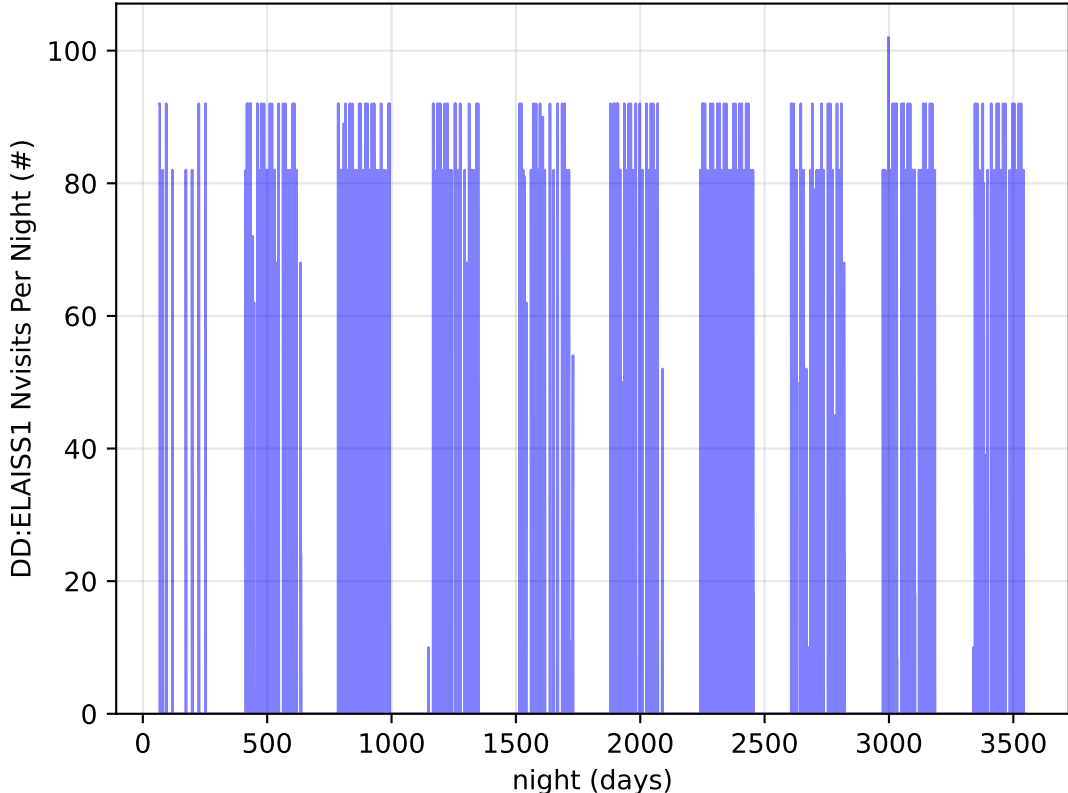
too_elab_heavy_r32_d3_gz_v3.4_10yrs all bands: DD:ELAISS1 Nvisits Per Night
