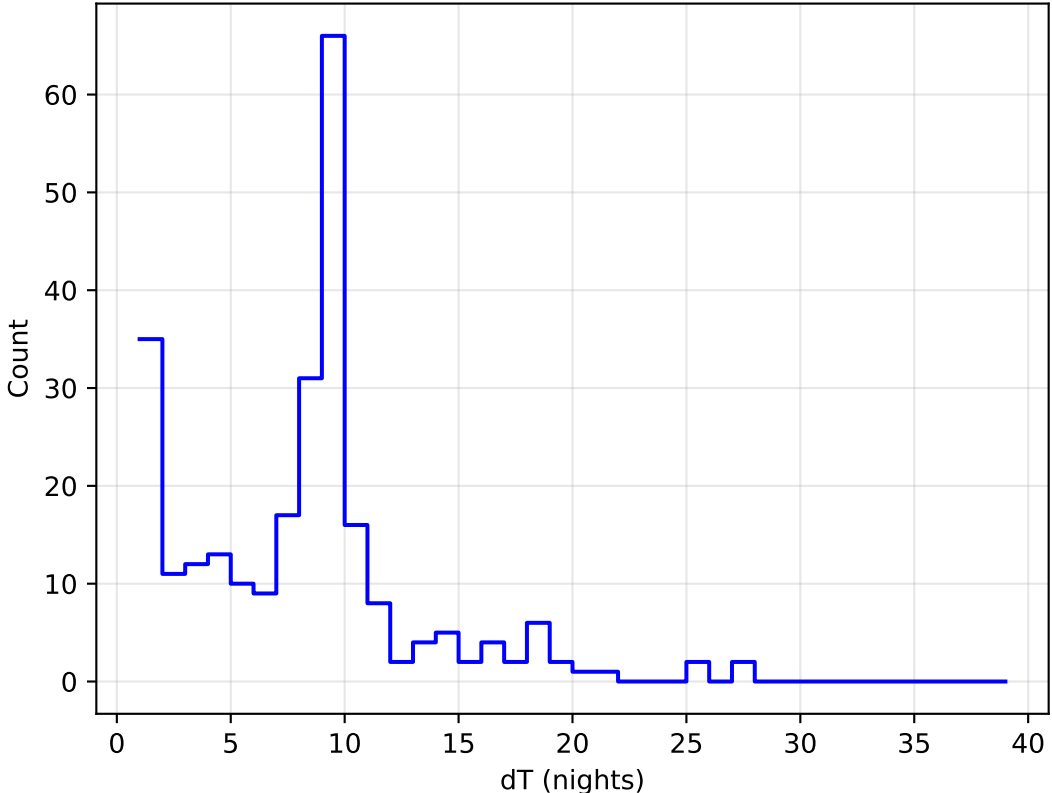
too_elab_heavy_r32_d3_gz_v3.4_10yrs all bands: DD:ELAISS1 Delta Nights Histogram
