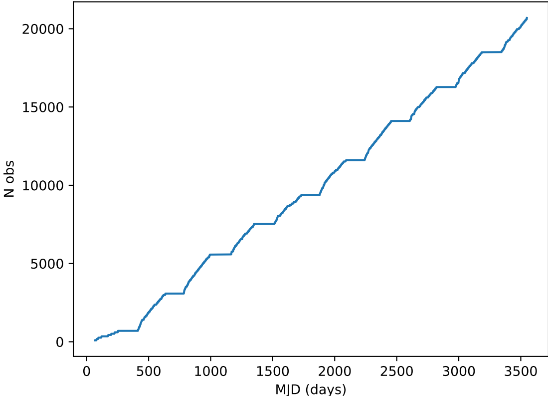
too_elab_heavy_r32_d3_gz_v3.4_10yrs all bands: DD:ELAISS1 Cumulative NVisits
