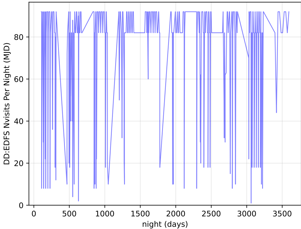
too_elab_heavy_r32_d3_gz_v3.4_10yrs all bands: DD:EDFS Nvisits Per Night
