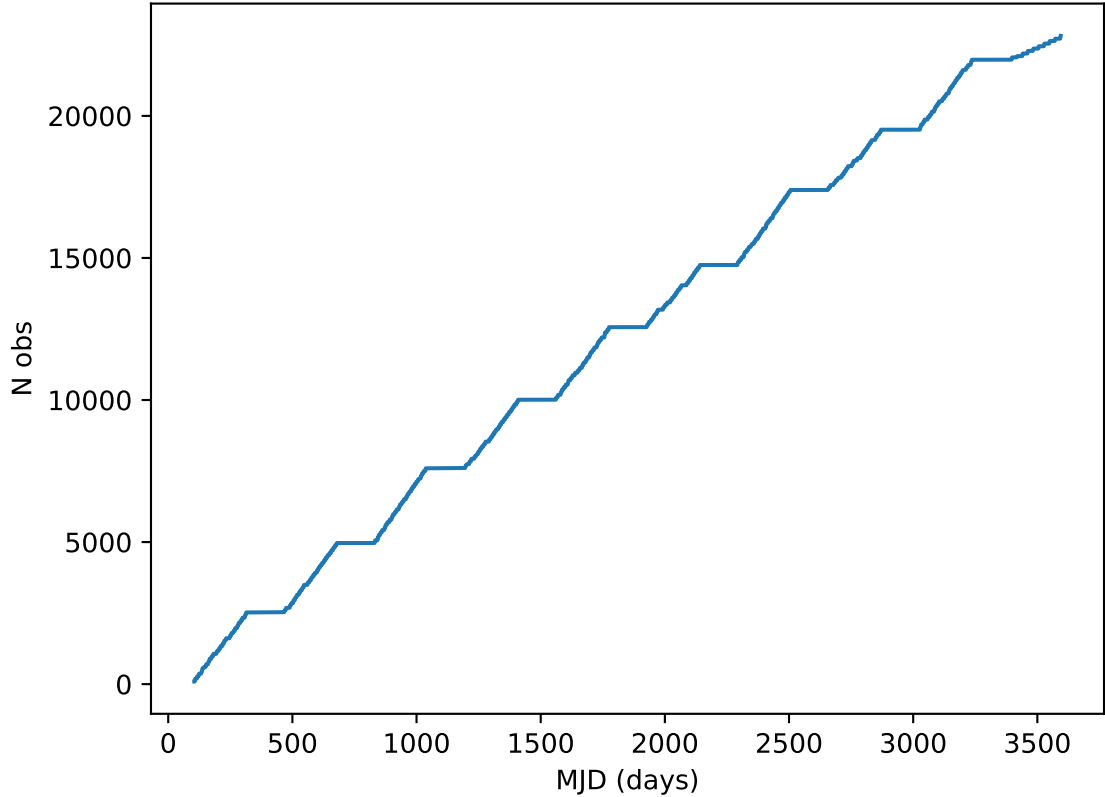
too_elab_heavy_r32_d3_gz_v3.4_10yrs all bands: DD:EDFS Cumulative NVisits
