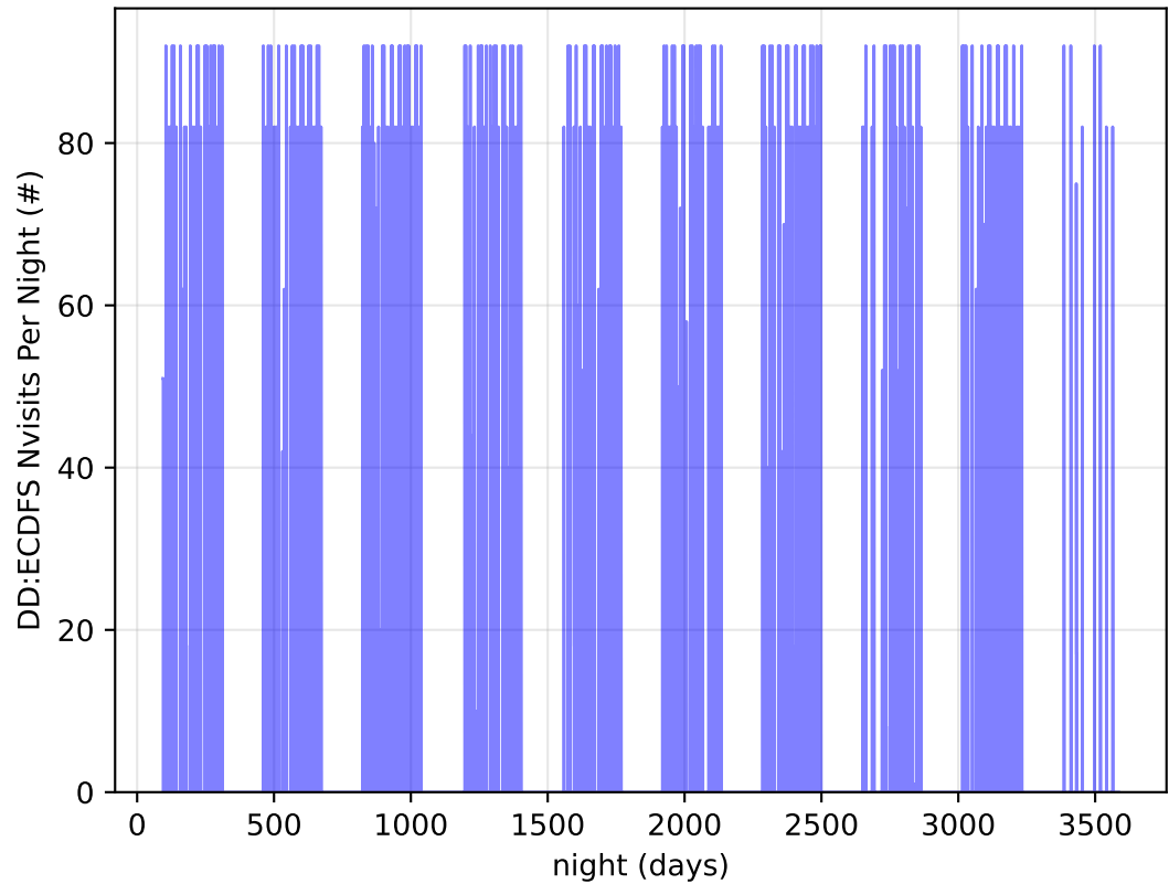
too_elab_heavy_r32_d3_gz_v3.4_10yrs all bands: DD:ECDFS Nvisits Per Night
