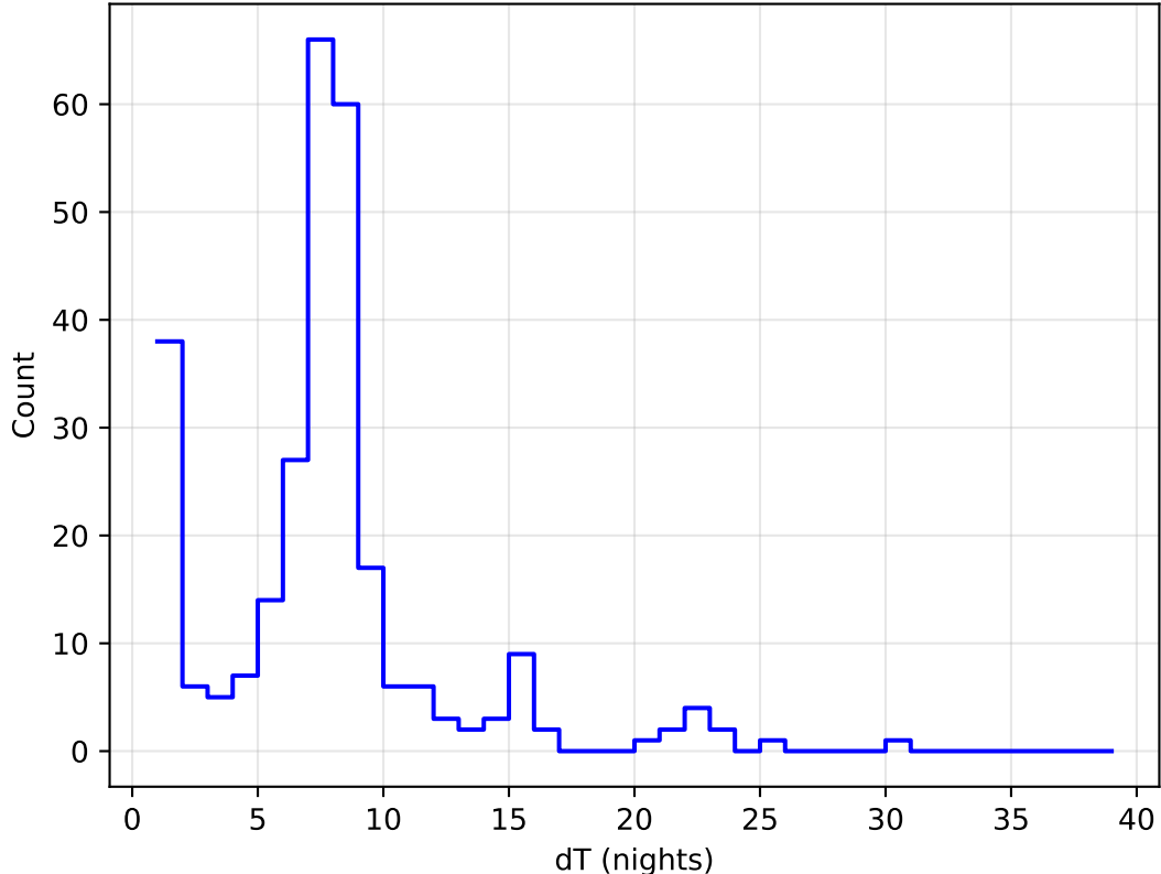
too_elab_heavy_r32_d3_gz_v3.4_10yrs all bands: DD:ECDFS Delta Nights Histogram
