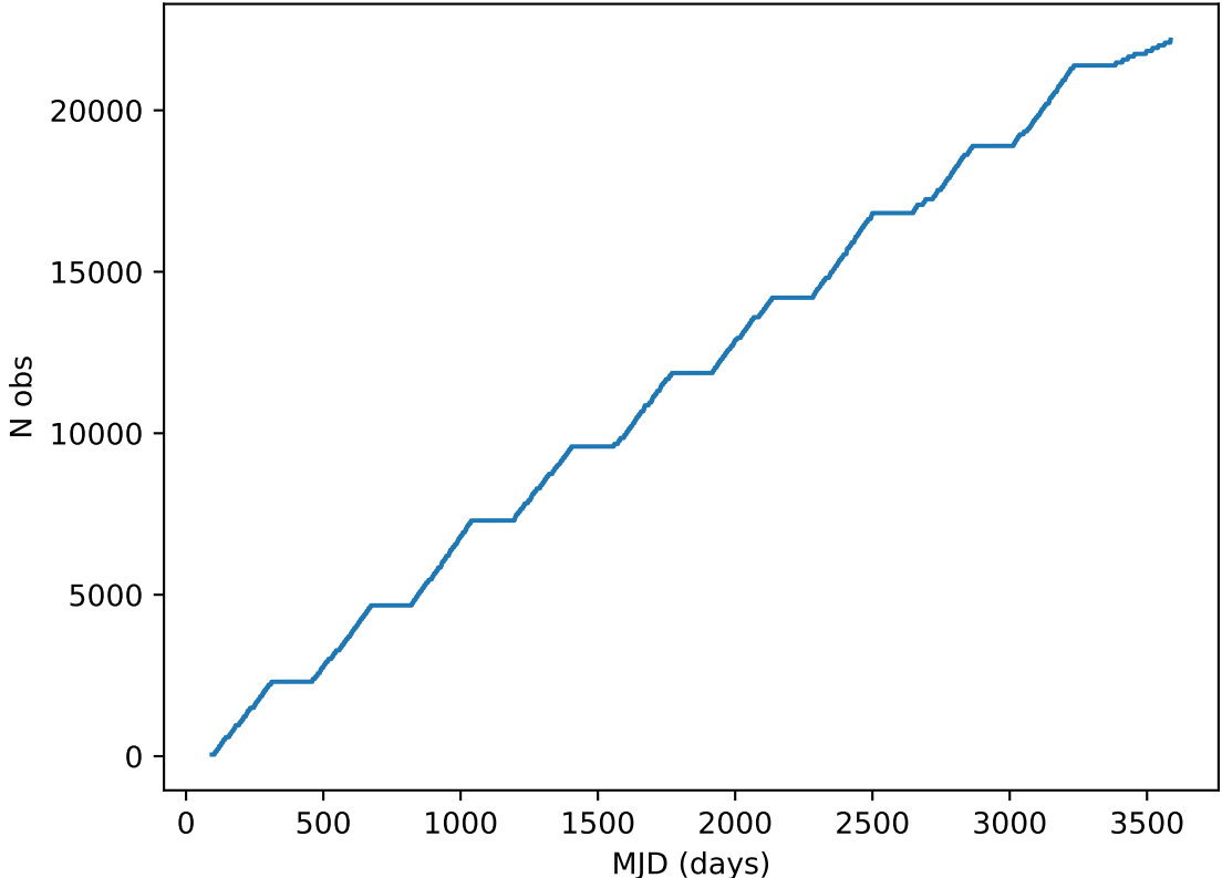
too_elab_heavy_r32_d3_gz_v3.4_10yrs all bands: DD:ECDFS Cumulative NVisits
