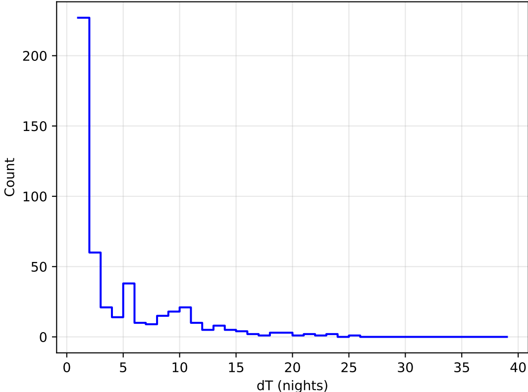
too_elab_heavy_r32_d3_gz_v3.4_10yrs all bands: DD: COSMOS Delta Nights Histogram
