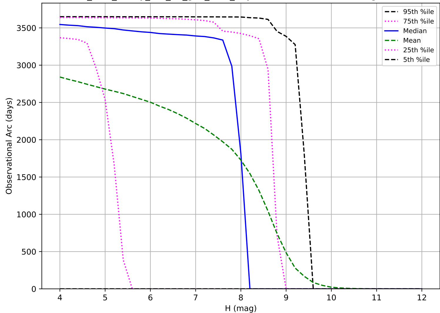
too_elab_heavy_r32_d3_griz_v3.4_10yrs: Observational Arc Length TNO
