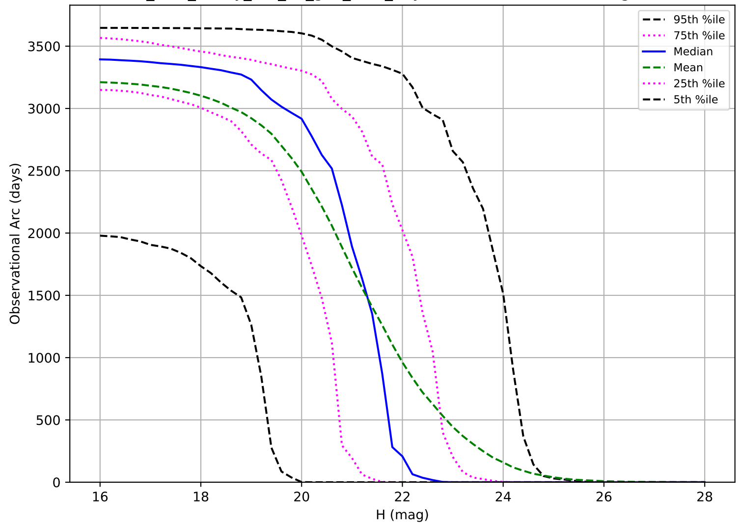
too_elab_heavy_r32_d3_griz_v3.4_10yrs: Observational Arc Length PHA
