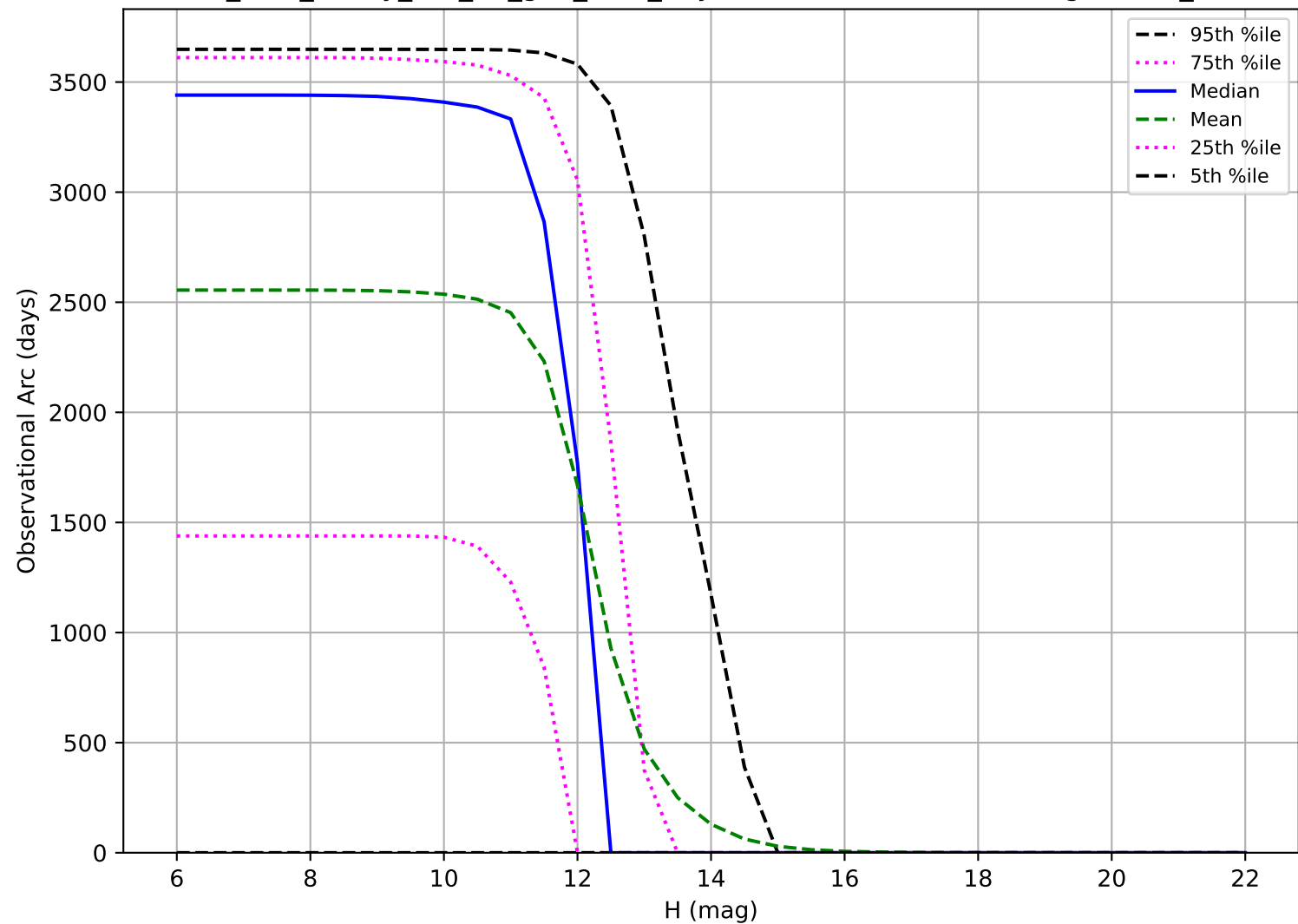
too_elab_heavy_r32_d3_griz_v3.4_10yrs: Observational Arc Length OCC_r20
