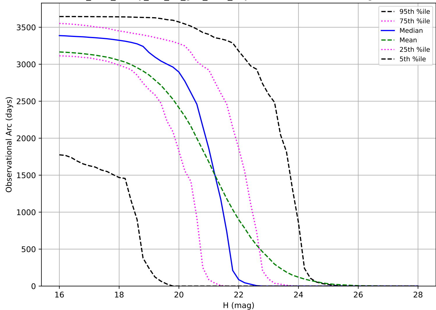
too_elab_heavy_r32_d3_griz_v3.4_10yrs: Observational Arc Length NEO
