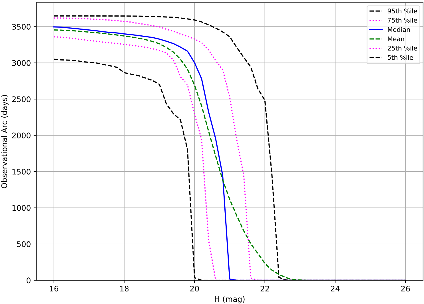
too_elab_heavy_r32_d3_griz_v3.4_10yrs: Observational Arc Length MBA
