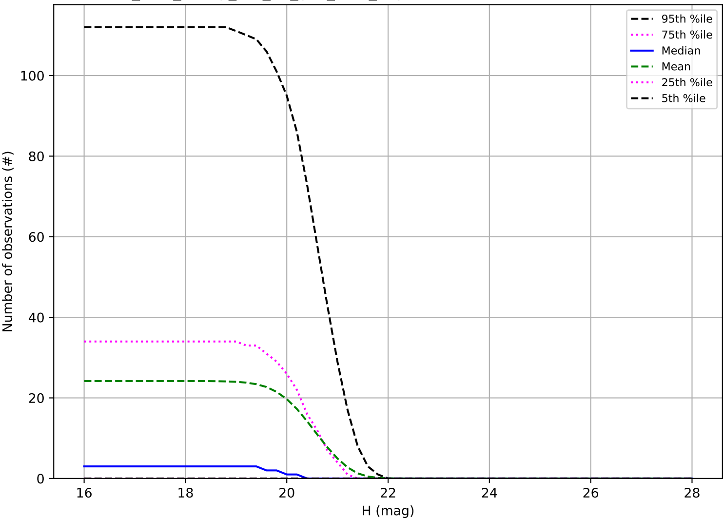
too_elab_heavy_r32_d3_griz_v3.4_10yrs: Number of observations Vatira
