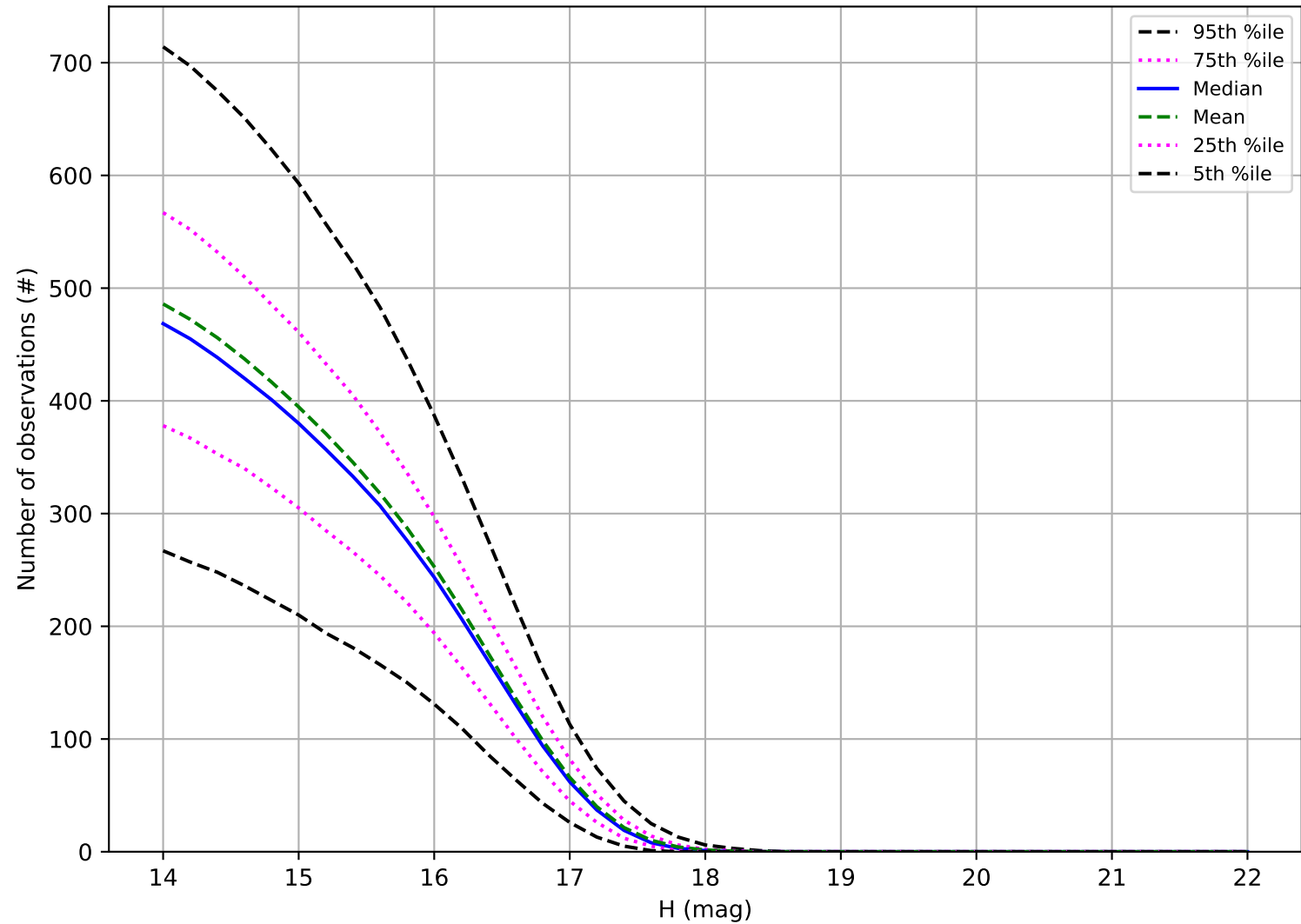
too_elab_heavy_r32_d3_griz_v3.4_10yrs: Number of observations Trojan
