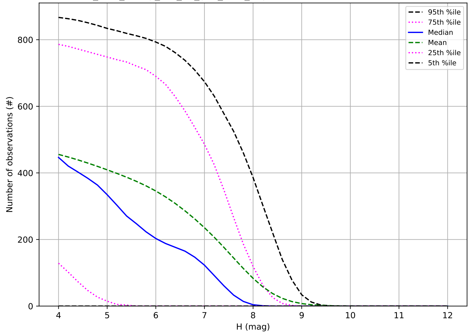
too_elab_heavy_r32_d3_griz_v3.4_10yrs: Number of observations TNO
