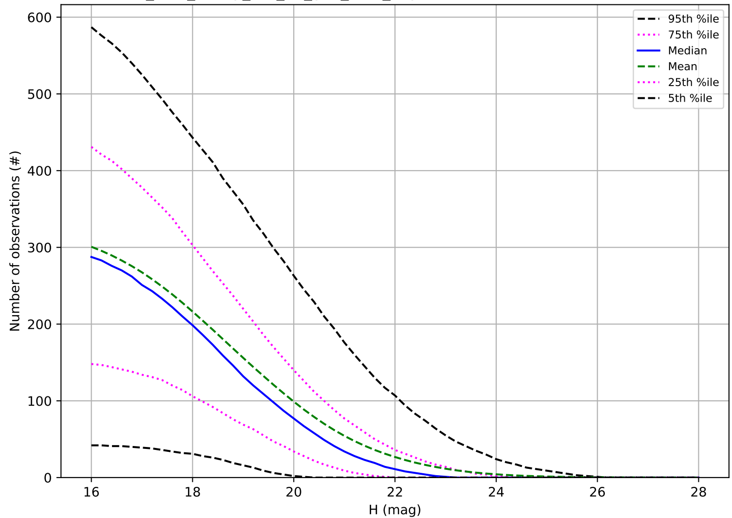
too_elab_heavy_r32_d3_griz_v3.4_10yrs: Number of observations PHA
