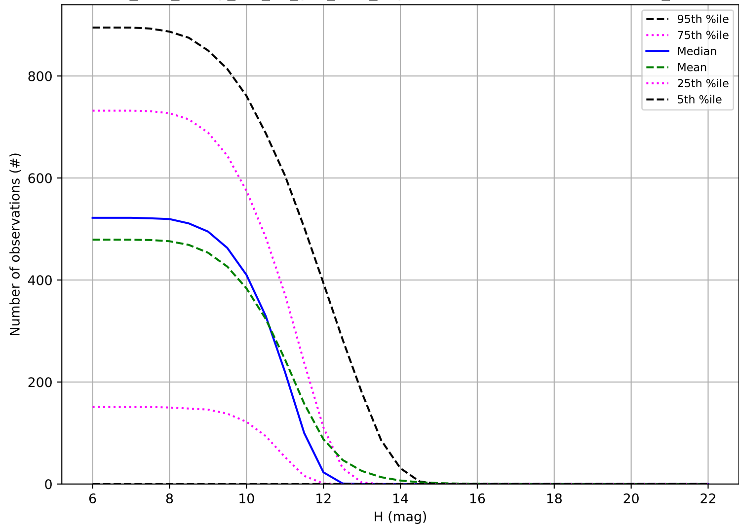
too_elab_heavy_r32_d3_griz_v3.4_10yrs: Number of observations OCC_r20
