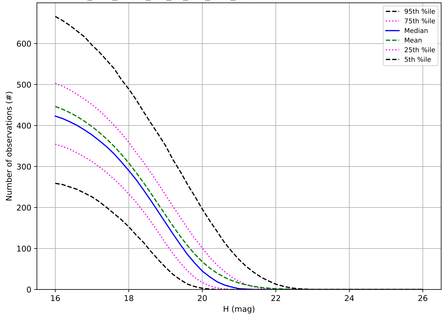
too_elab_heavy_r32_d3_griz_v3.4_10yrs: Number of observations MBA
