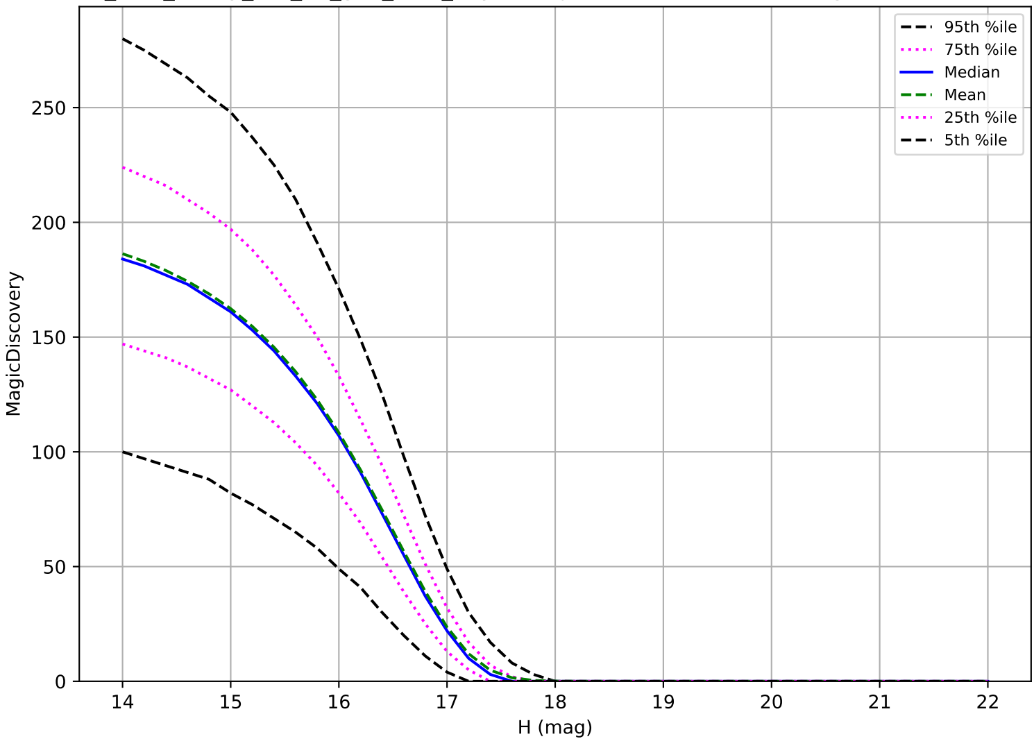
too_elab_heavy_r32_d3_griz_v3.4_10yrs: Trojan 6 detections in 60 nights detection loss
