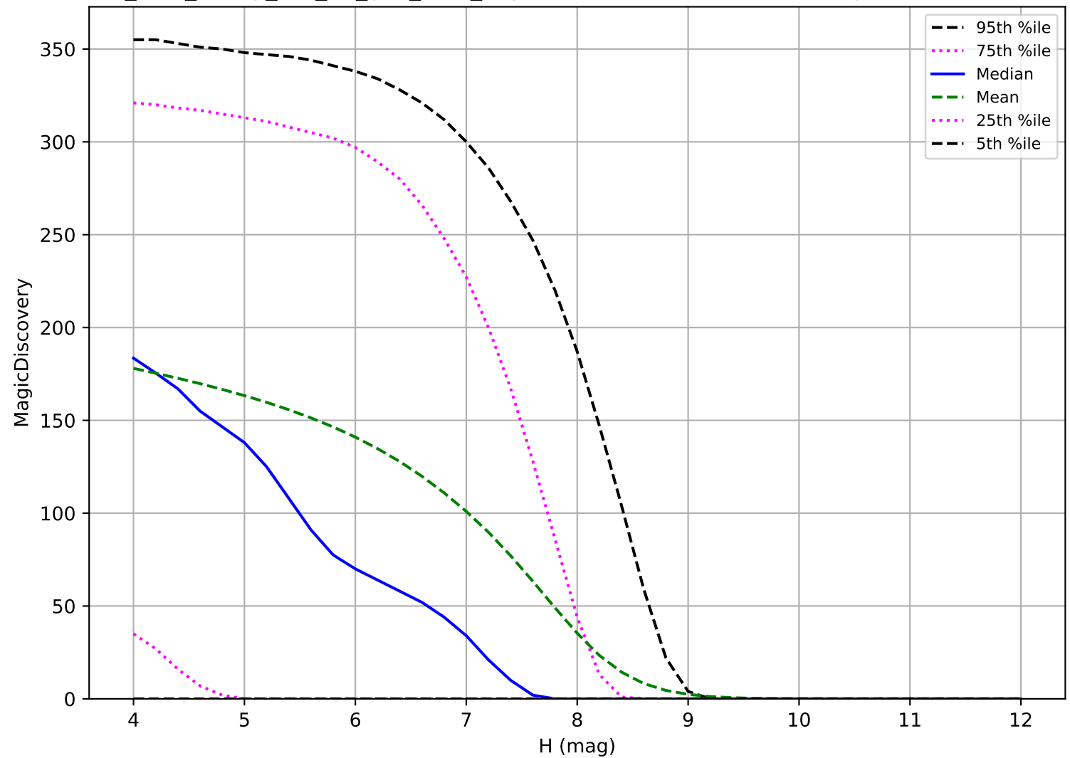
too_elab_heavy_r32_d3_griz_v3.4_10yrs: TNO 6 detections in 60 nights detection loss
