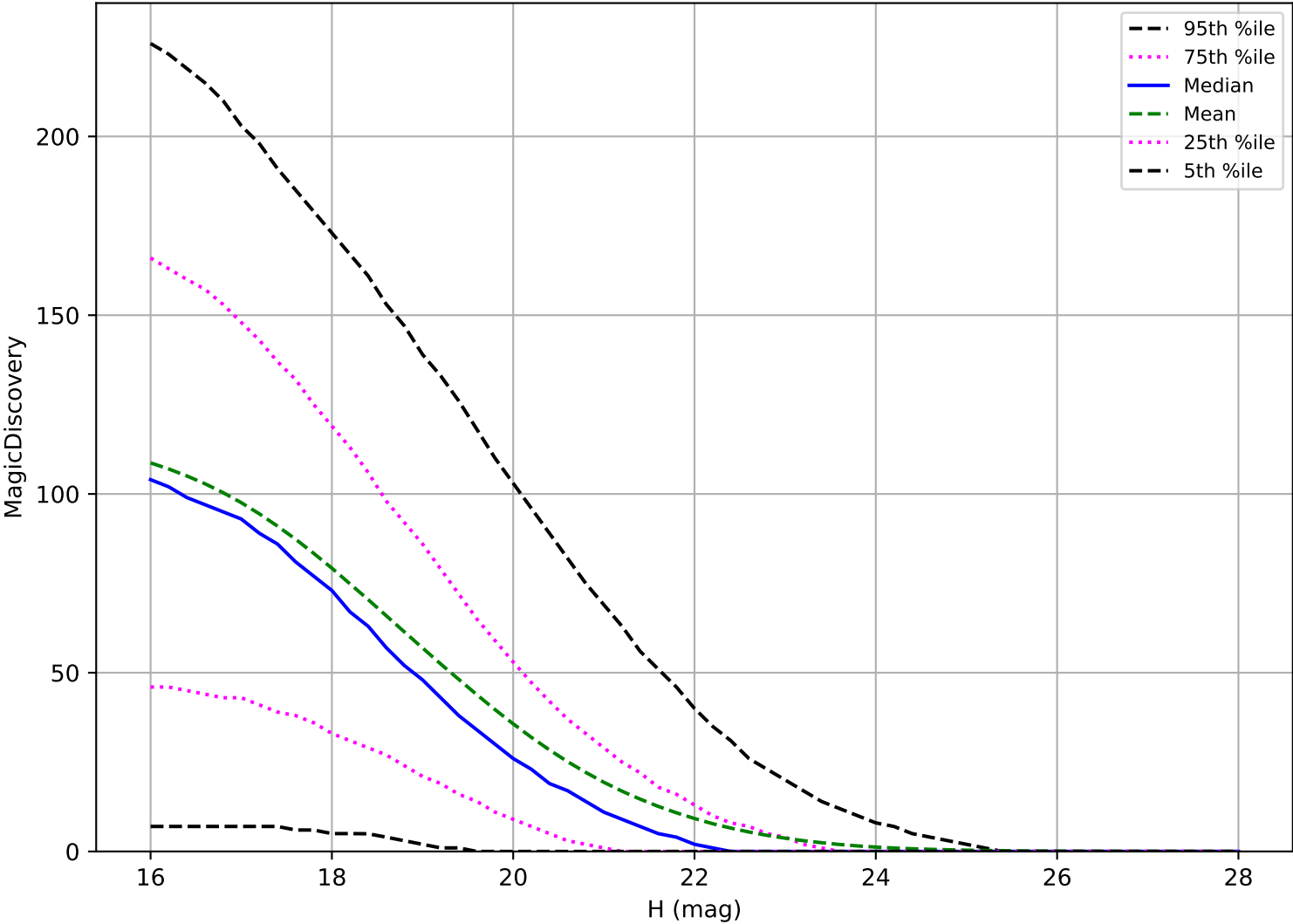
too_elab_heavy_r32_d3_griz_v3.4_10yrs: PHA 6 detections in 60 nights detection loss
