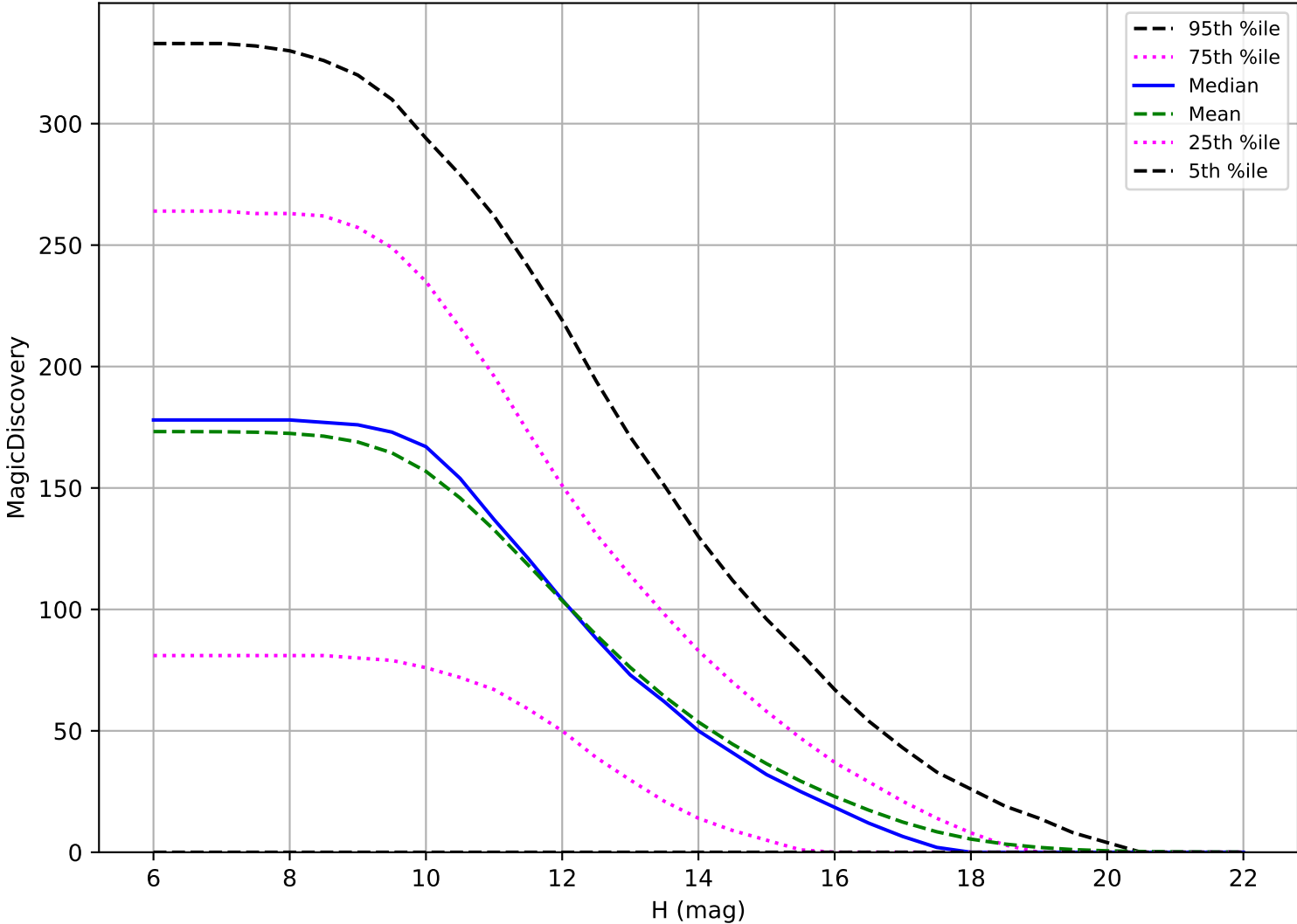
too_elab_heavy_r32_d3_griz_v3.4_10yrs: OCC_r5 6 detections in 60 nights detection loss
