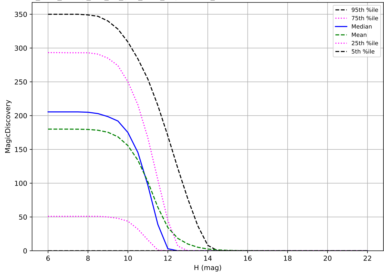
too_elab_heavy_r32_d3_griz_v3.4_10yrs: OCC_r20 6 detections in 60 nights detection loss
