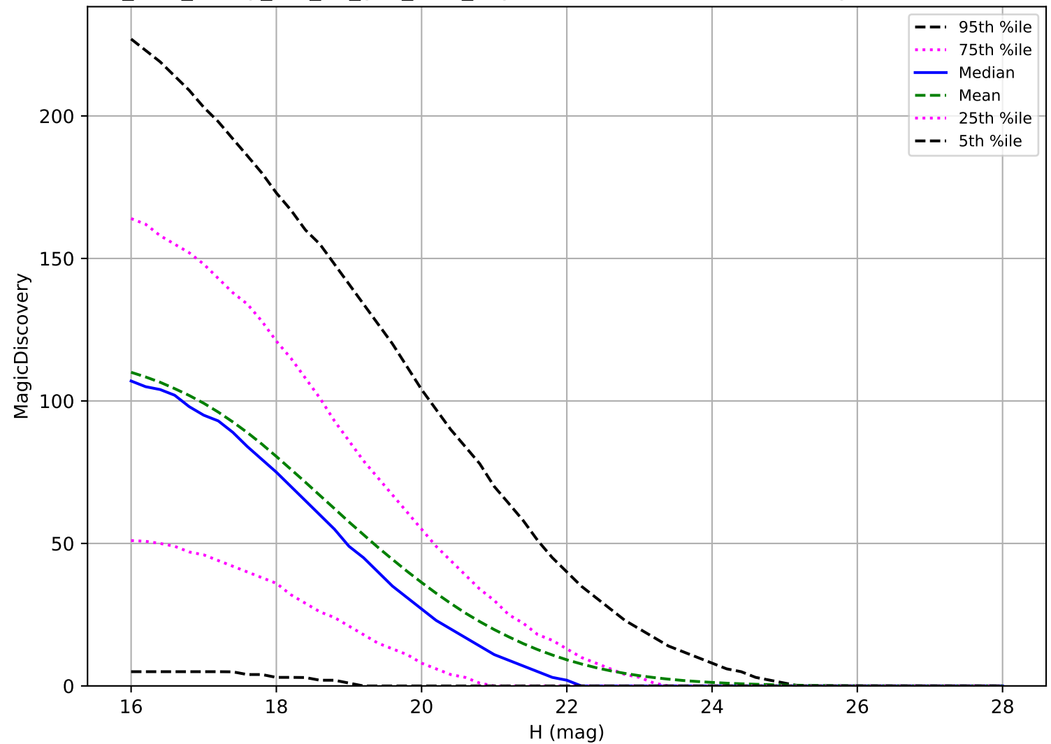
too_elab_heavy_r32_d3_griz_v3.4_10yrs: NEO 6 detections in 60 nights detection loss
