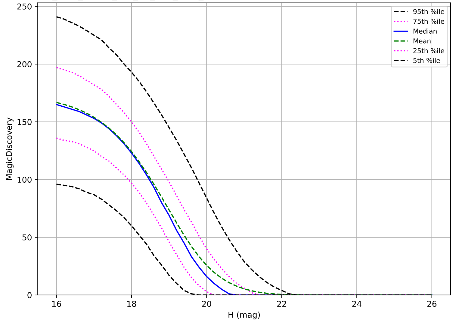
too_elab_heavy_r32_d3_griz_v3.4_10yrs: MBA 6 detections in 60 nights detection loss
