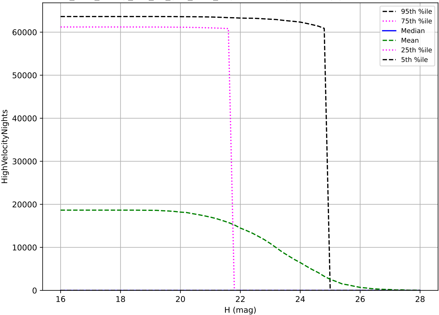
too_elab_heavy_r32_d3_griz_v3.4_10yrs: NEO High velocity pair detection loss
