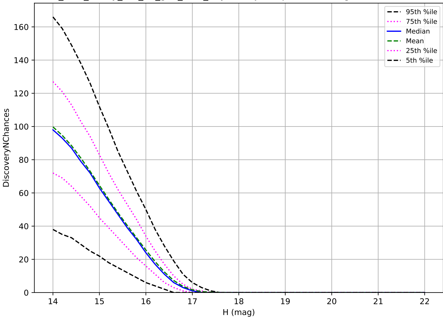
too_elab_heavy_r32_d3_griz_v3.4_10yrs: Trojan 3 pairs in 15 nights detection loss
