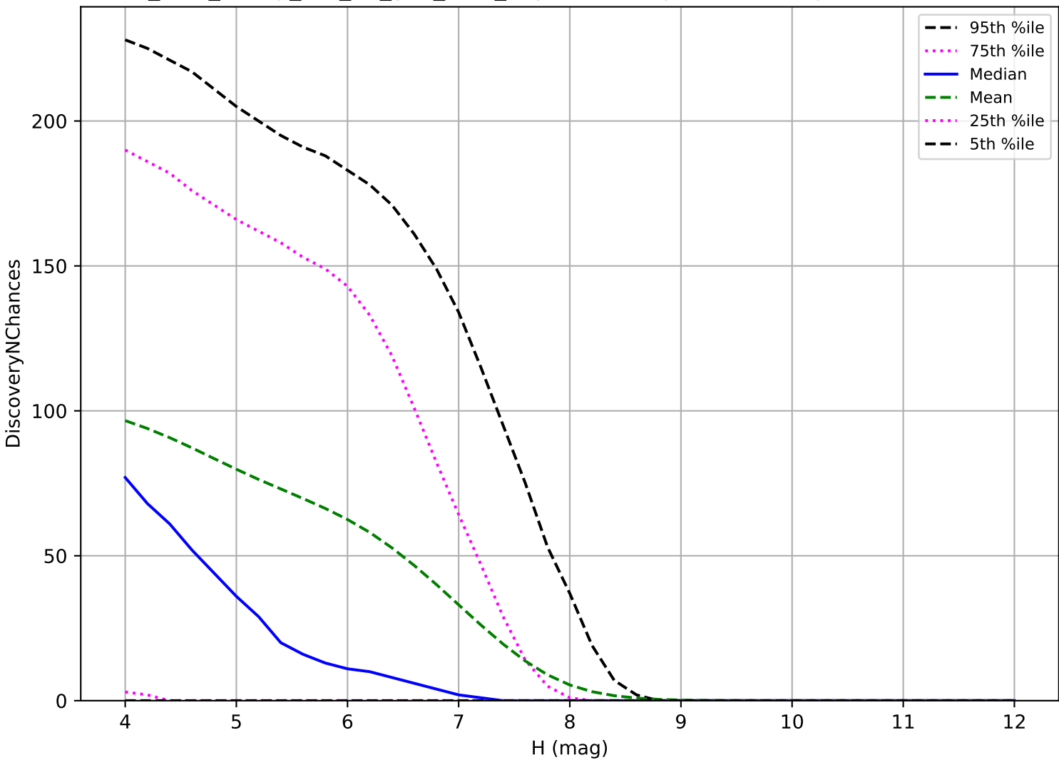
too_elab_heavy_r32_d3_griz_v3.4_10yrs: TNO 3 pairs in 15 nights detection loss
