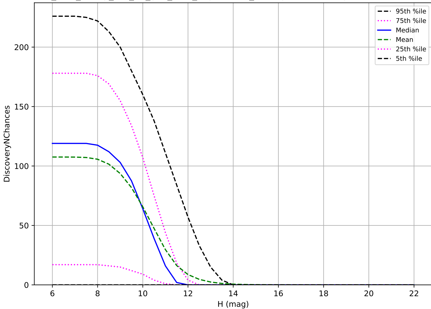
too_elab_heavy_r32_d3_griz_v3.4_10yrs: OCC_r20 3 pairs in 15 nights detection loss
