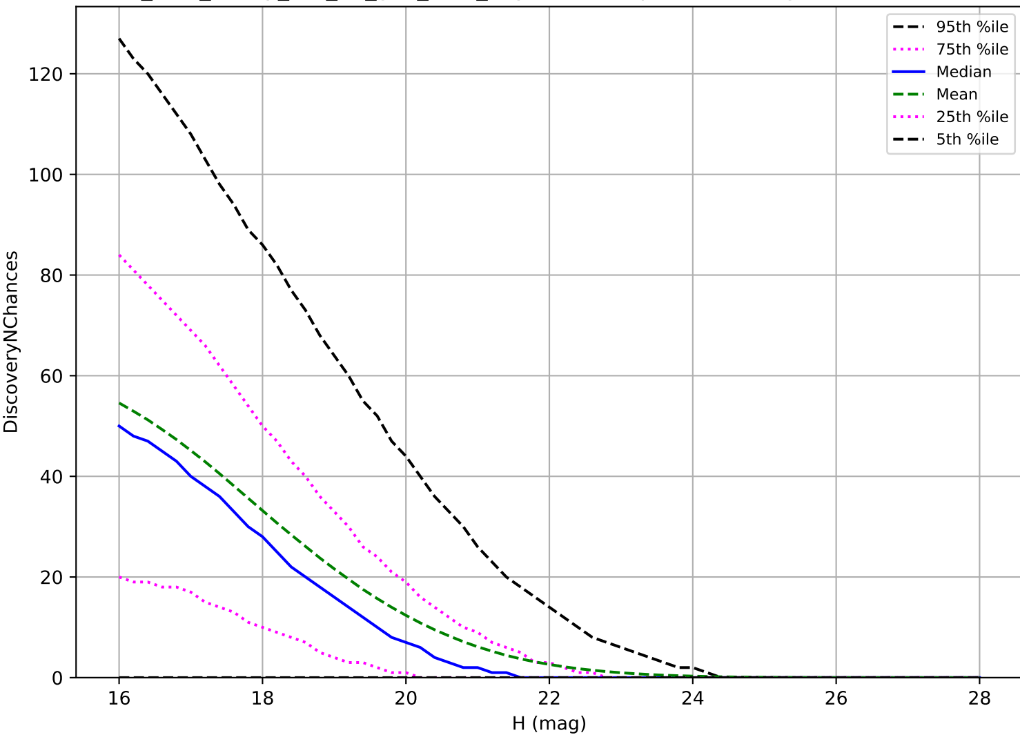
too_elab_heavy_r32_d3_griz_v3.4_10yrs: NEO 3 pairs in 15 nights detection loss
