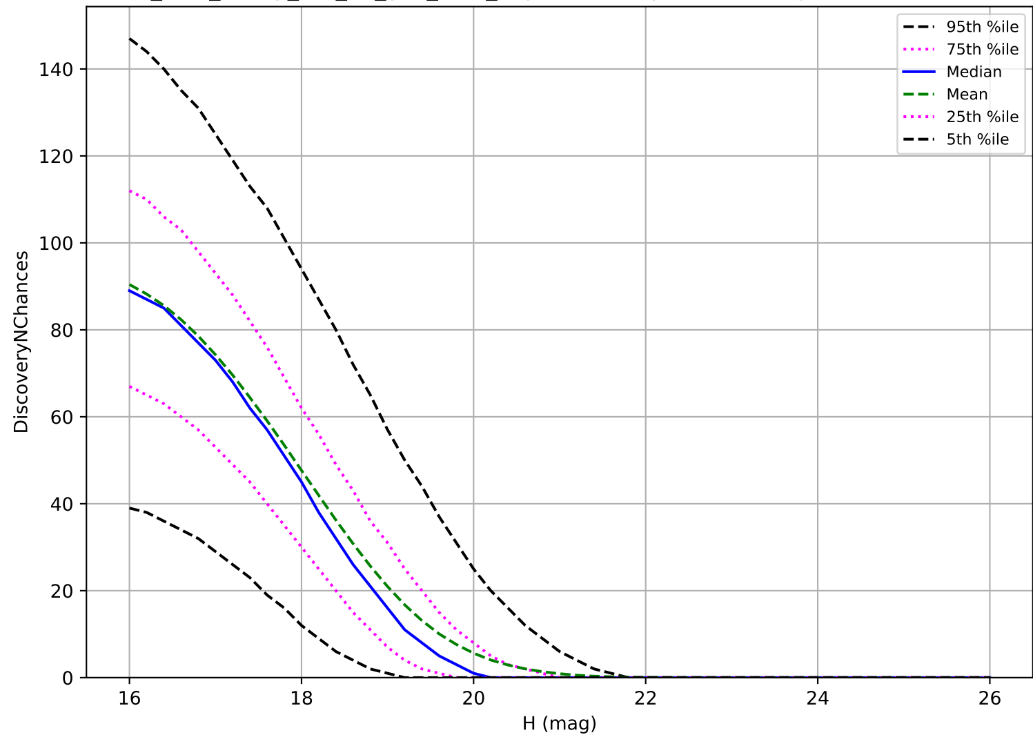
too_elab_heavy_r32_d3_griz_v3.4_10yrs: MBA 3 pairs in 15 nights detection loss
