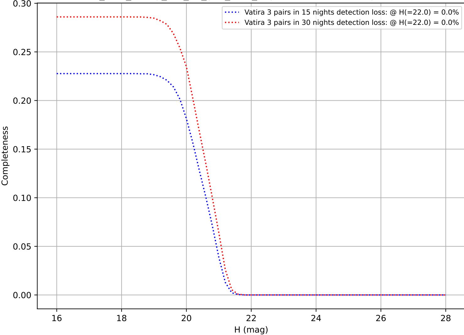
too_elab_heavy_r32_d3_griz_v3.4_10yrs: DifferentialCompleteness
