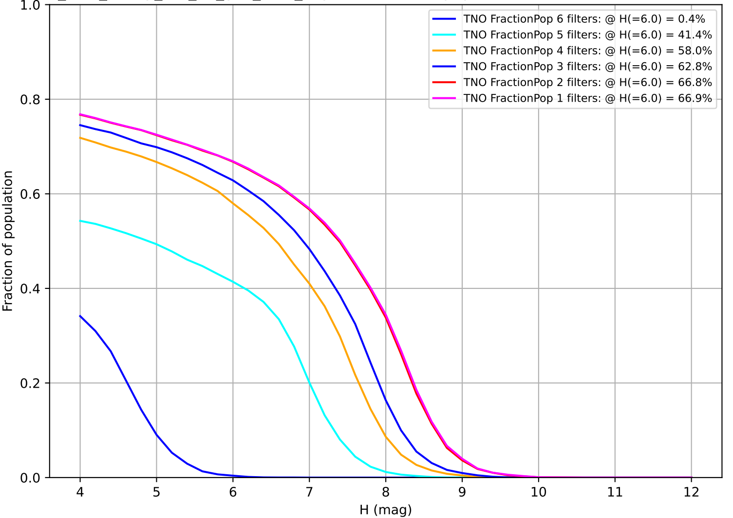
too_elab_heavy_r32_d3_griz_v3.4_10yrs: Fraction of population with colors in X filters TNO
