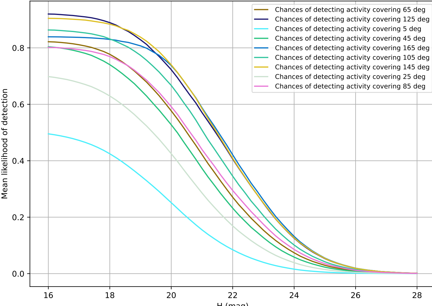
too elab heavy r32 d3 griz v3.4 10yrs PHA
